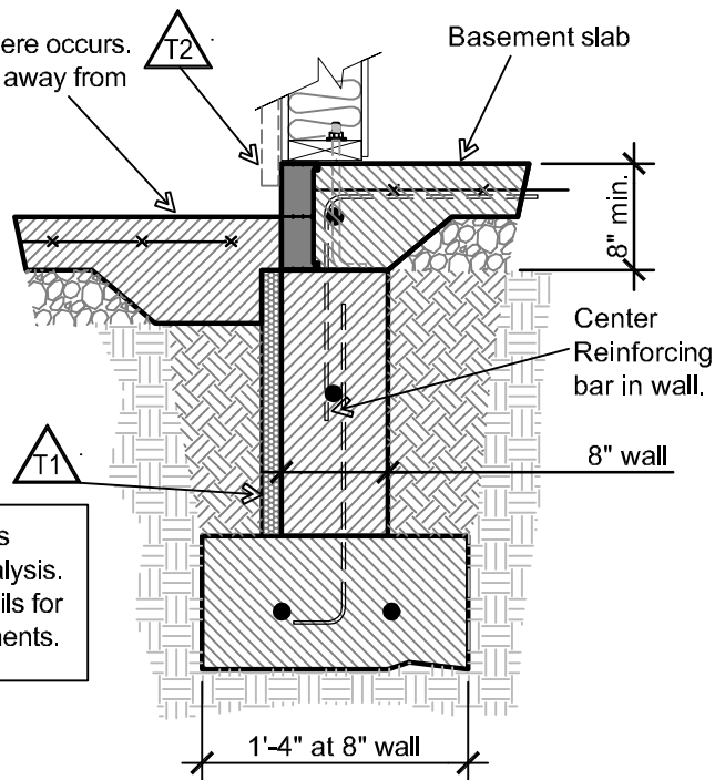
DET F4 WALK-OUT BASEMENT @ EXTERIOR PATIO TRADITIONAL SLAB EDGE
